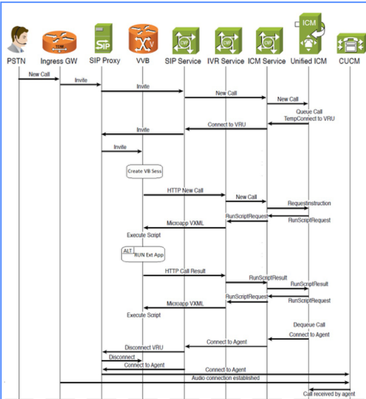
Unified CVP Comprehensive SIP Call Flow Ladder Diagram
