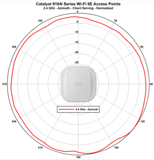
Catalyst 9164 2.4-GHz client serving radio
