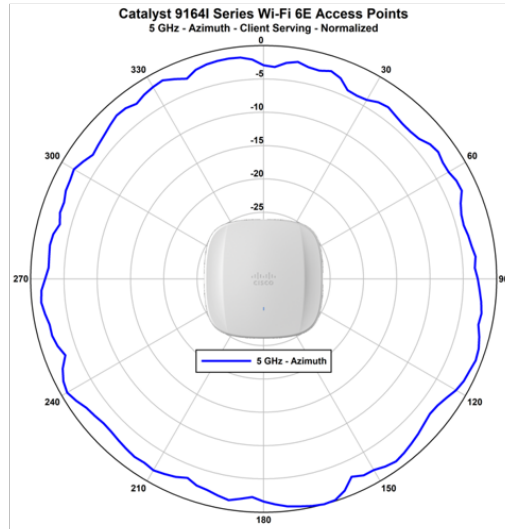
Catalyst 9164 5-GHz client serving radio
