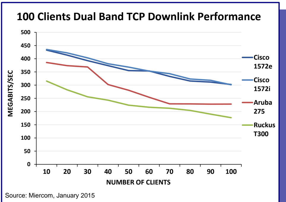
Figure 1: High Client Density Performance
