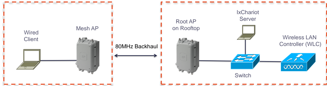
Figure 9: Outdoor Mesh Network Diagram
