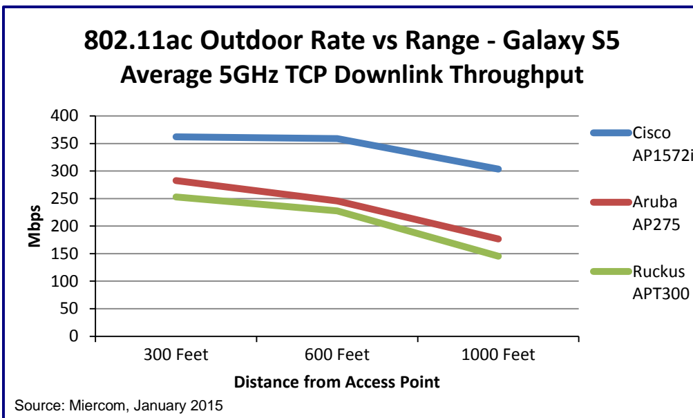
Figure 4: Galaxy S5 Throughput at 300, 600 and 1,000 Feet
