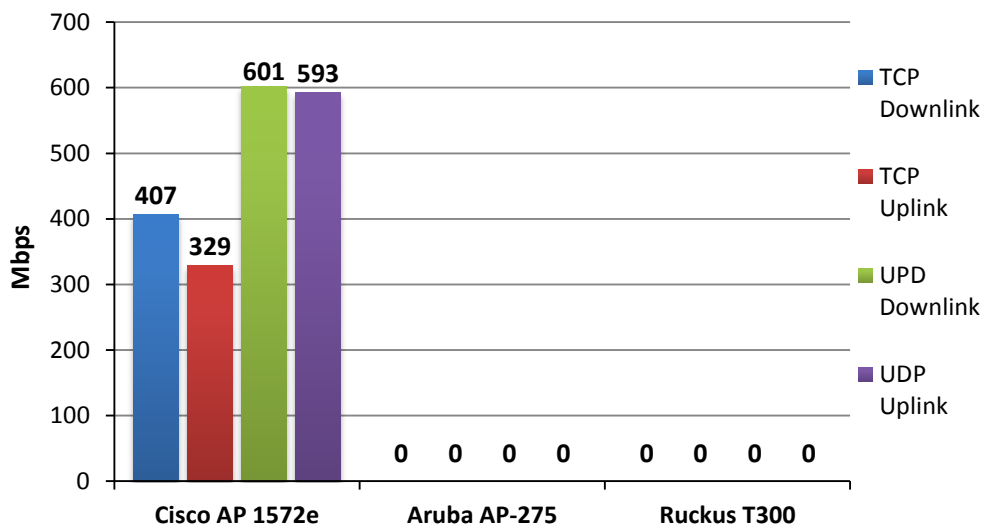
Figure 10: Outdoor 802.11ac Mesh Backhaul Performance
