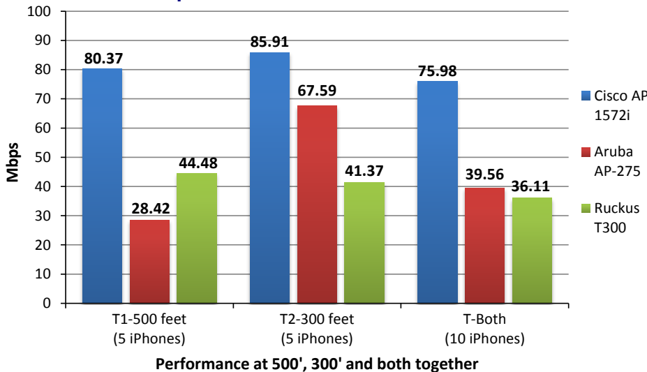
Figure 8: 802.11ac Outdoor Performance and Consistency iPhone 6 phones on two tables at 500' and 300'
