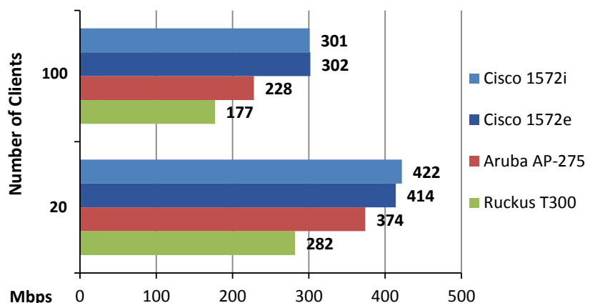
Figure 11: High Client Density Test Results Summary Average per-client TCP downlink throughput (Mbps)
