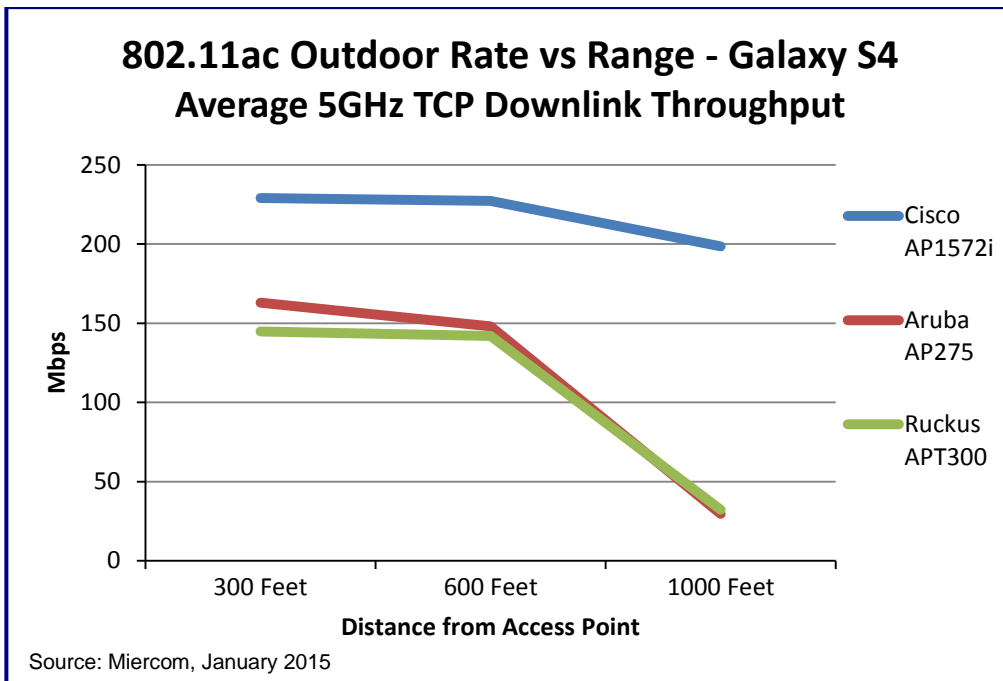
Figure 3: Galaxy S4 Throughput at 300, 600 and 1,000 Feet
